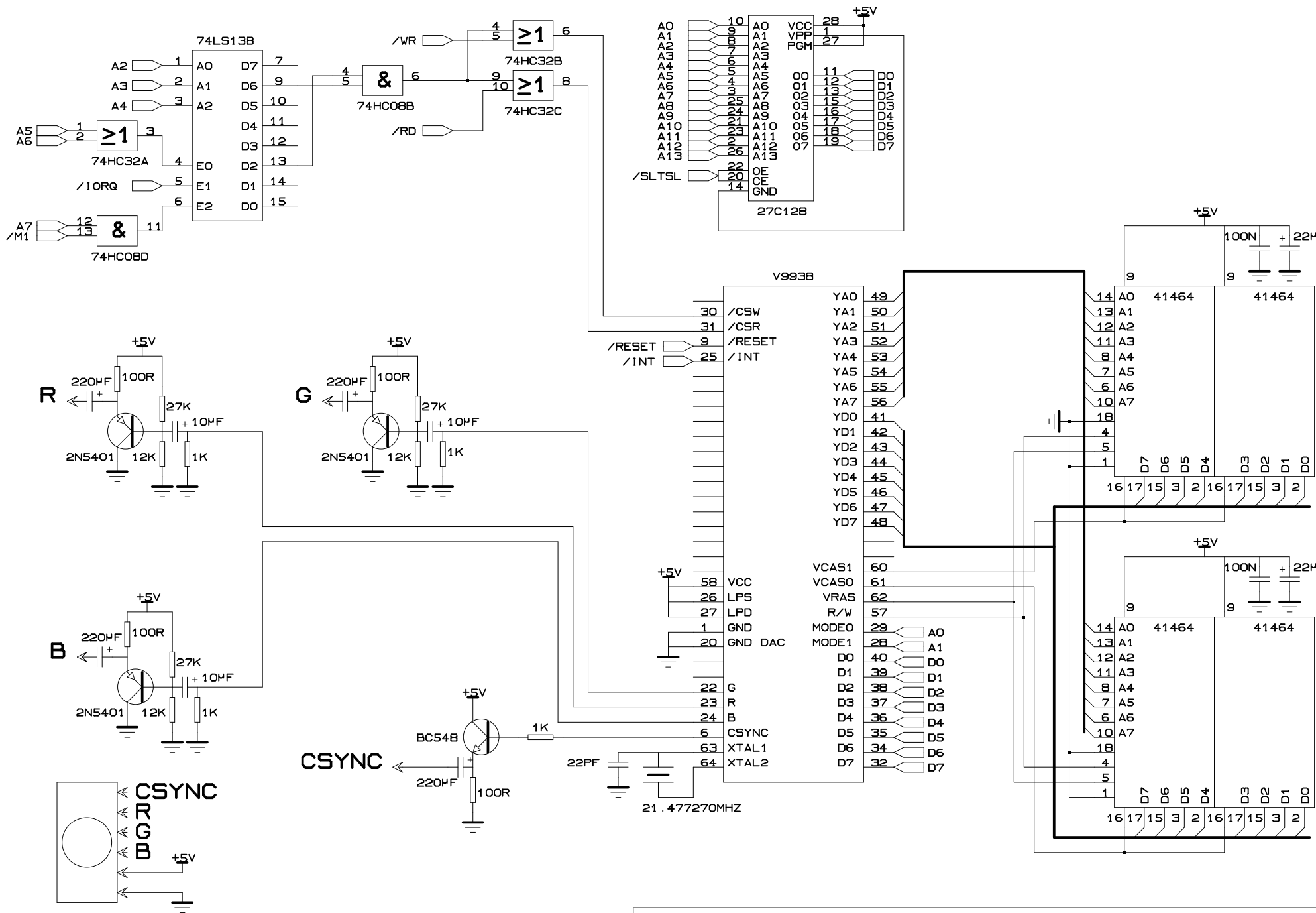
EXTENSION MSX2 128KO VRAM - RGB TRANSISTORS
